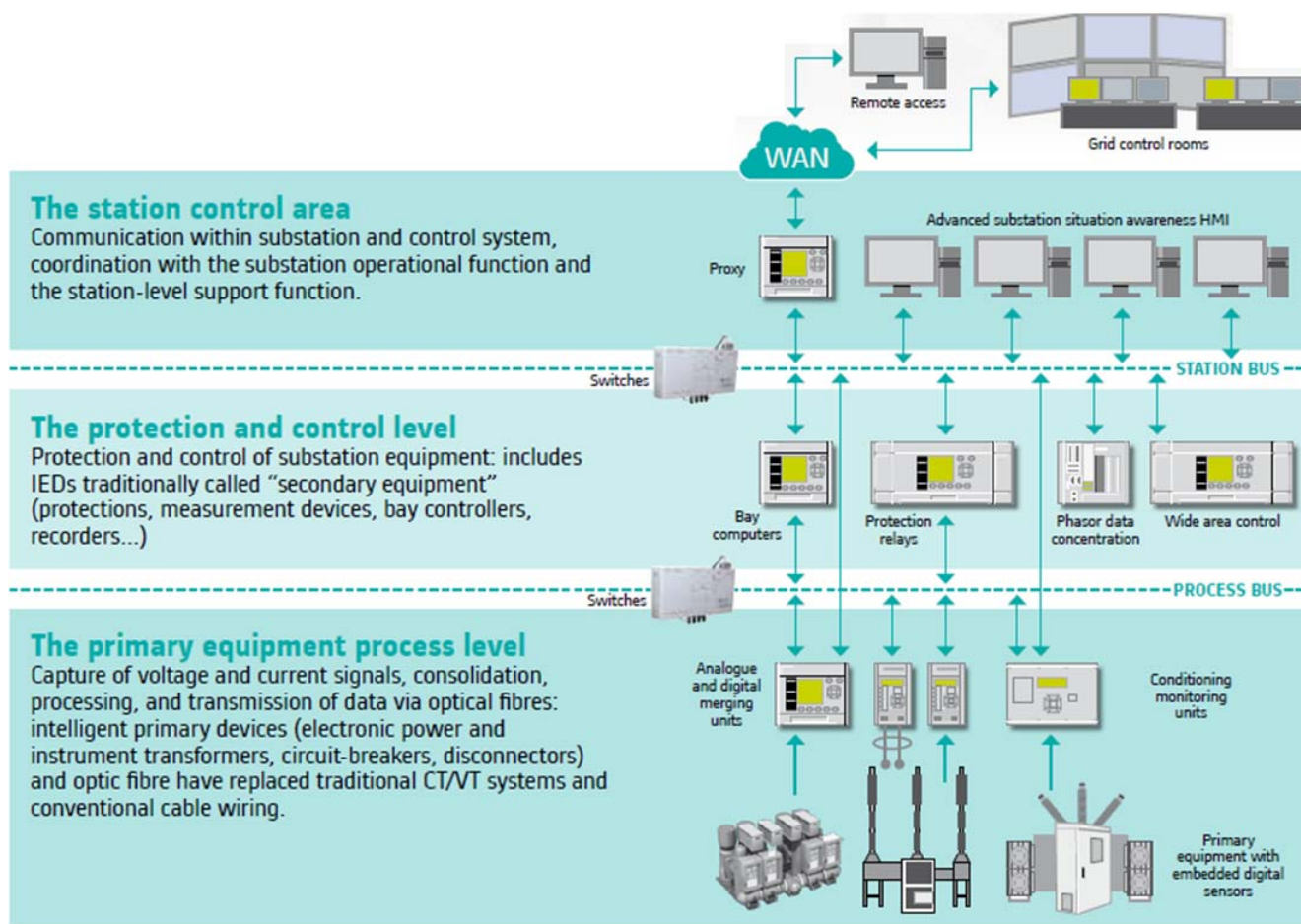
Fig. 1 – Architecture levels in a digital substation
