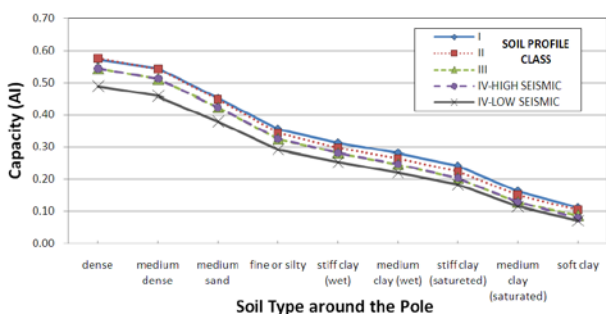
Figure.4: Capacity curve for tension pole (9 meter)
