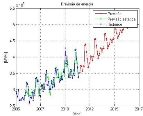
Figure 4 – Residential Energy Consumption Forecast
