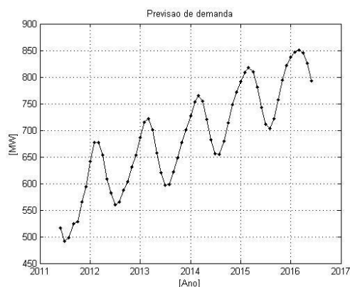
Figure 7 – Commercial Demand Forecast
