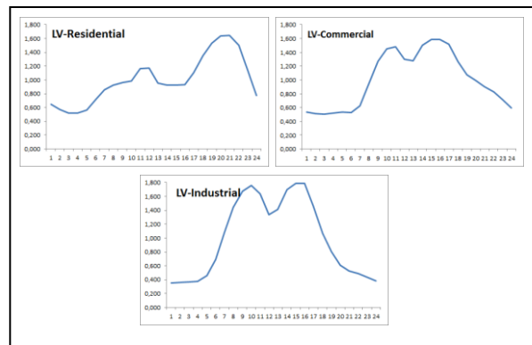
Figure 1 – Consumers Typical Curves for residential, industrial and commercial demand.
