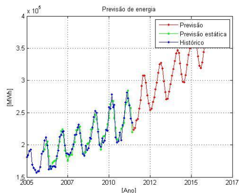
Figure 6 – Commercial Energy Consumption Forecast
