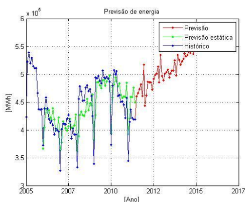
Figure 8 – Industrial Energy Consumption Forecast
