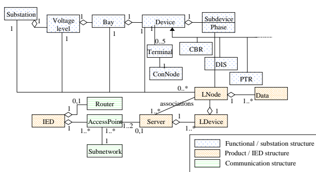
Fig. 5 Simplified UML diagram of the substation configuration language
