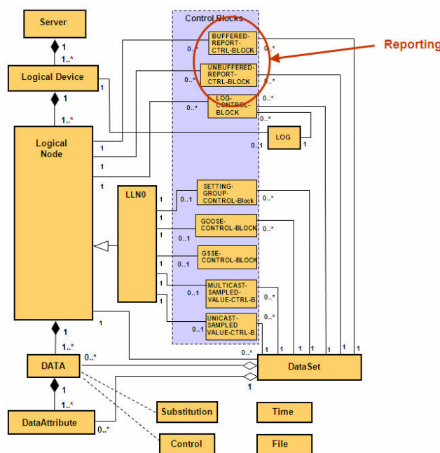
Fig. 3 IEC 61850 reporting services
