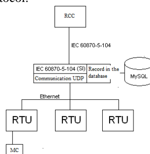
Figure 3: Protocol RTU <-> concentrator
