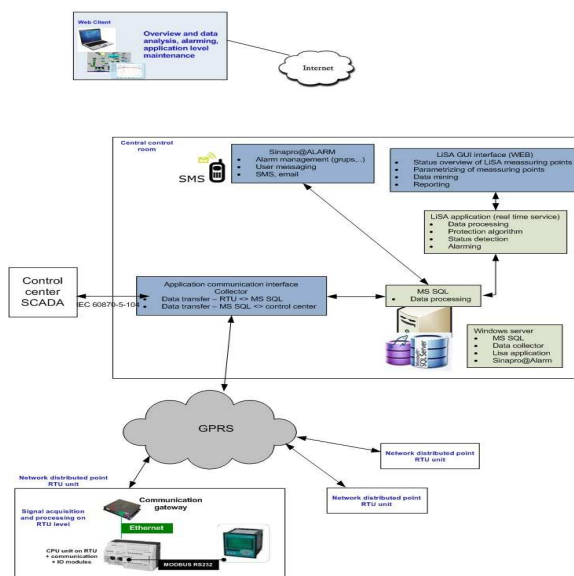
Figure 4: Overview of the system
