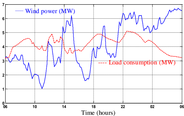
Figure5. Wind power and load consumption profile
