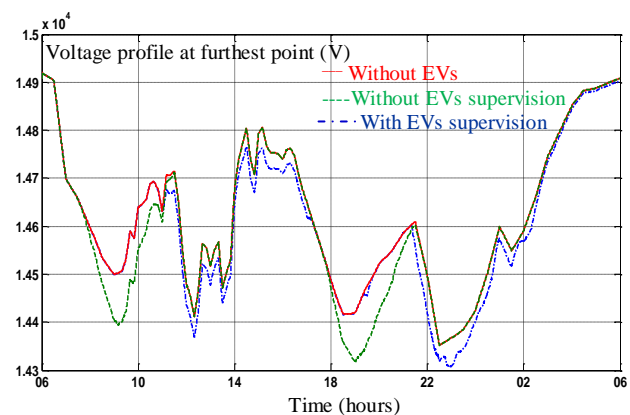
Figure8. Voltage profile at furthest point
