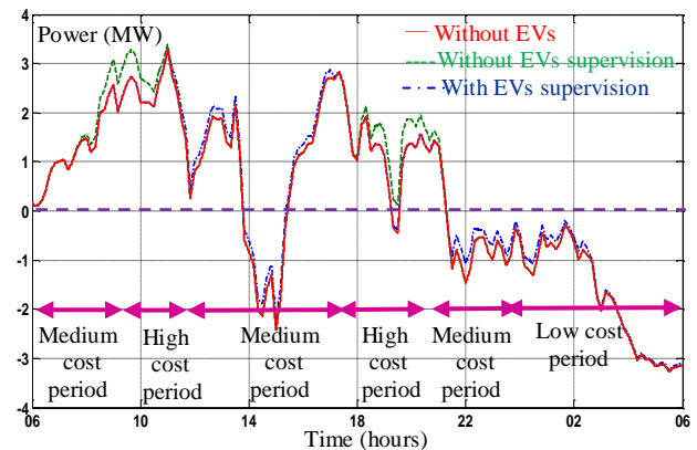
Figure6. Measured power at substation
