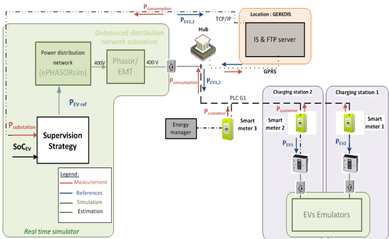
Figure4. Test platform overview
