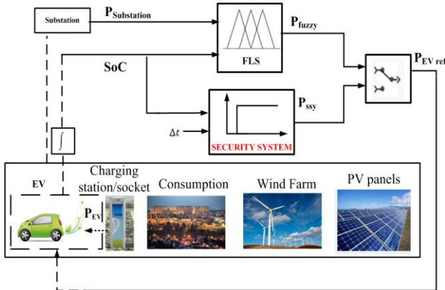
Figure 1. Supervision Strategy Architecture
