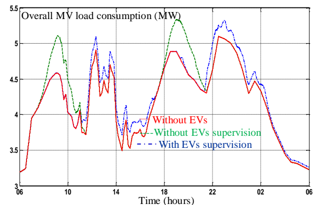
Figure7. Overall MV load consumption
