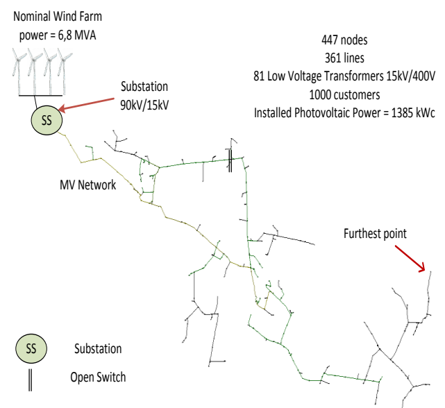
Figure 2. Medium Voltage network specifications
