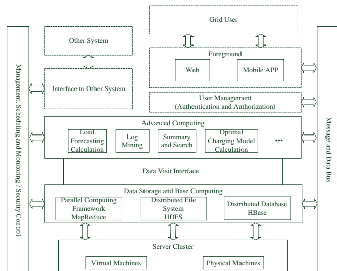
Figure 4. Multi-level feedback queue optimized charging system architecture
