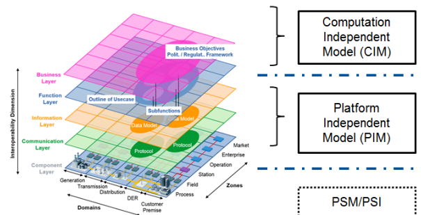
Figure 1 - The SGAM and its mapping with the upper two layers of the MDA
