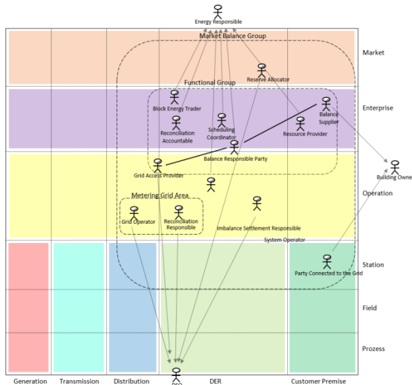
Figure 32 Roles and Domains mapped onto the SGAM Business Layer
