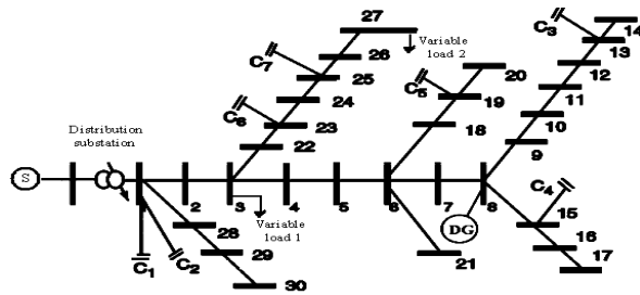
Figure.2 : The one-line diagram of 30-bus radial test feeder
