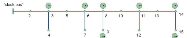
Figure 1. 15 node radial networks used for G&E load flow test.
