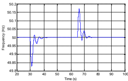
Fig. 8.a: frequency
