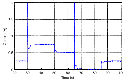
Fig. 9.c: Currents (in HTA lines)
