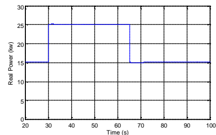
Fig. 7: P_{load2} , required power from the load2
