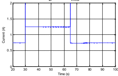
Fig. 8.c: Currents (in HTA lines)
