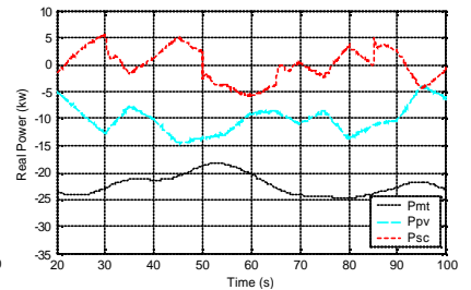
Fig. 9.e: Powers from sources inside the MG
