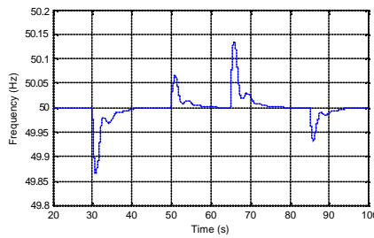
Fig. 9.a: frequency
