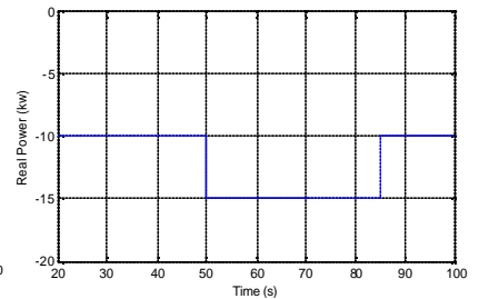
Fig. 9.d: P_{mg\_dso\_ref}
