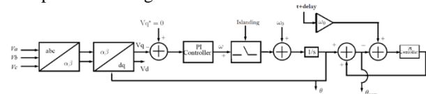
Fig. 4. Block diagram for Independent timing based methodology for deriving phase angle information
