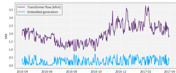
Fig. 2: Example of embedded generation with transformer flow
