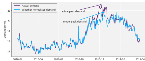
Fig. 6: Annual peak demand from actual demand and weather-normalised demand
